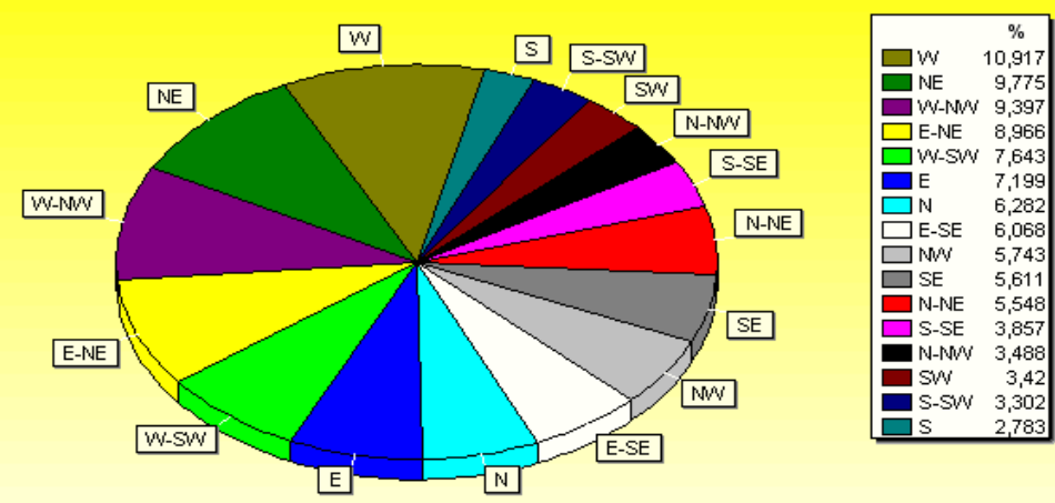
Distribution Wind direction Year 2004
